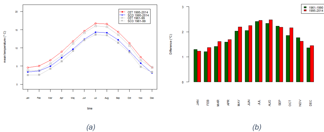
Figure 1. Comparative changes in mean temperature between CET and SMT, decomposed by month
