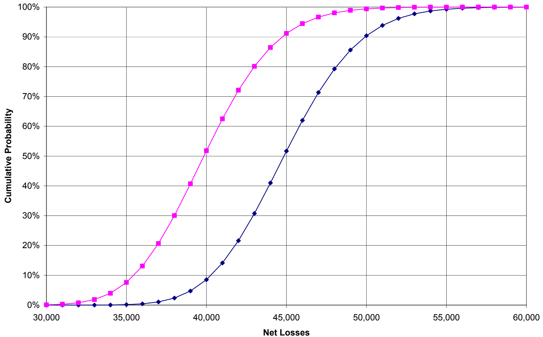
Graph 2) Variability of Net Losses Lognormal Approximation
