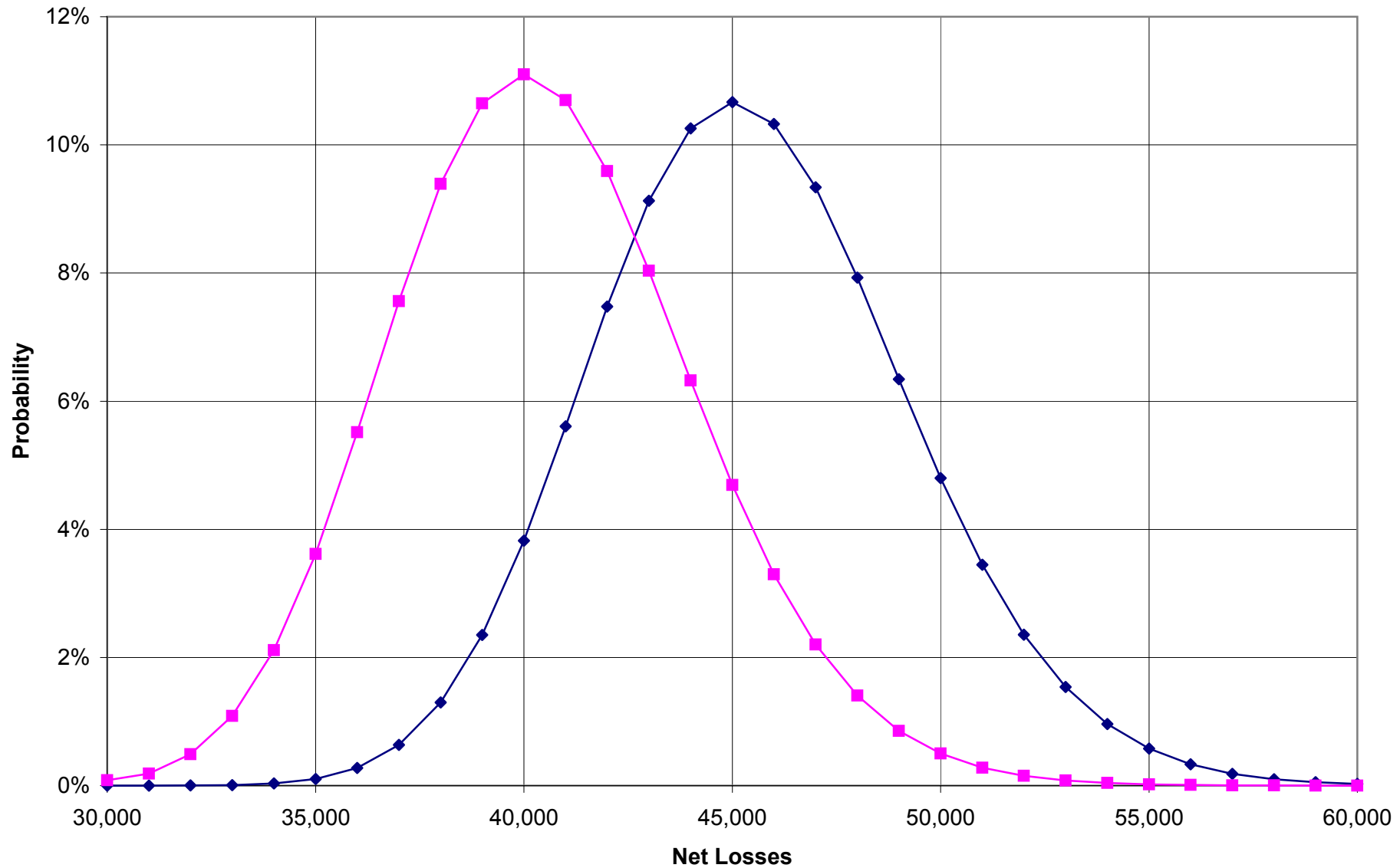
Graph 1) Variability of Net Losses Lognormal Approximation
