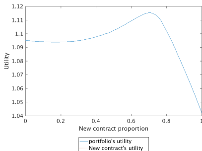
Figure: The composition of optimal portfolio for term of T = 12 . r_f = 0.04 , g = 0.02 , \mu = 0.1 , \sigma = 0.2 .
