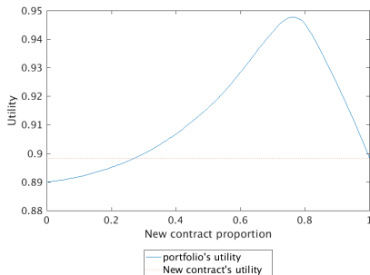
Figure: The composition of optimal portfolio for term of T = 10 . r_f = 0.04 , g = 0.02 , \mu = 0.1 , \sigma = 0.2 .
