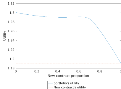
Figure: The composition of optimal portfolio for term of T = 14 . r_f = 0.04 , g = 0.02 , \mu = 0.1 , \sigma = 0.2 .
